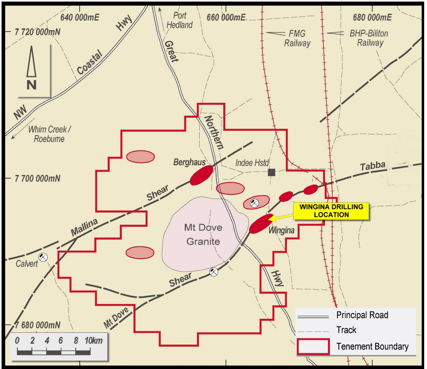
Figure 1 –Wingina Prospect Location Map
