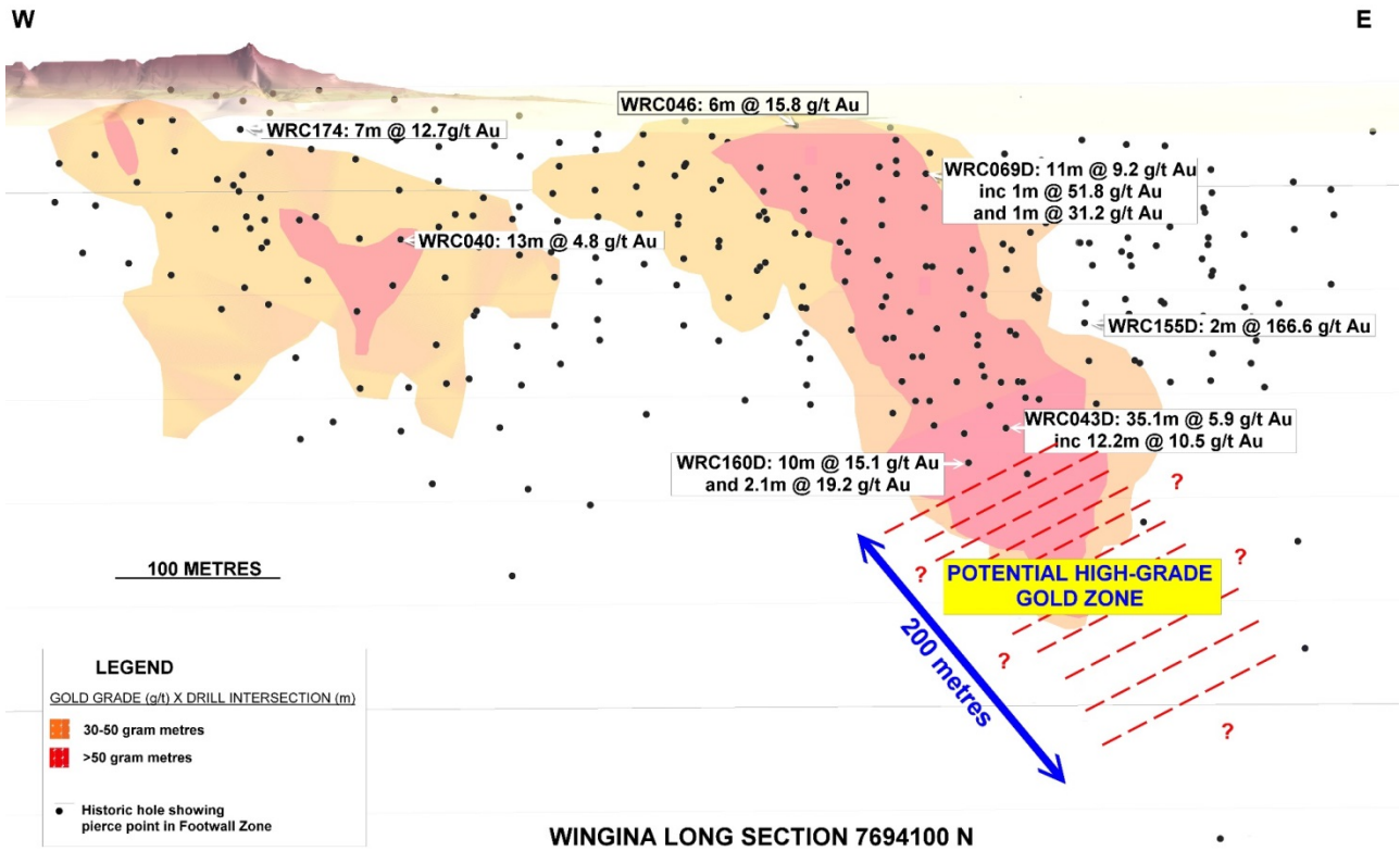
Figure 2: The Wingina Prospect Showing Potential High-Grade Gold Target
